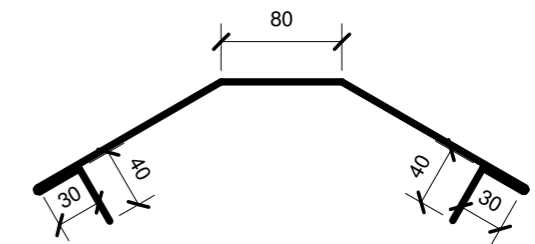
UNDER RIDGING OPTION 1
