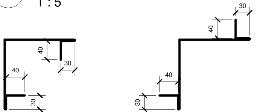
EXTERNAL CORNER
