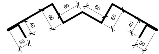
UNDER RIDGING OPTION 2
