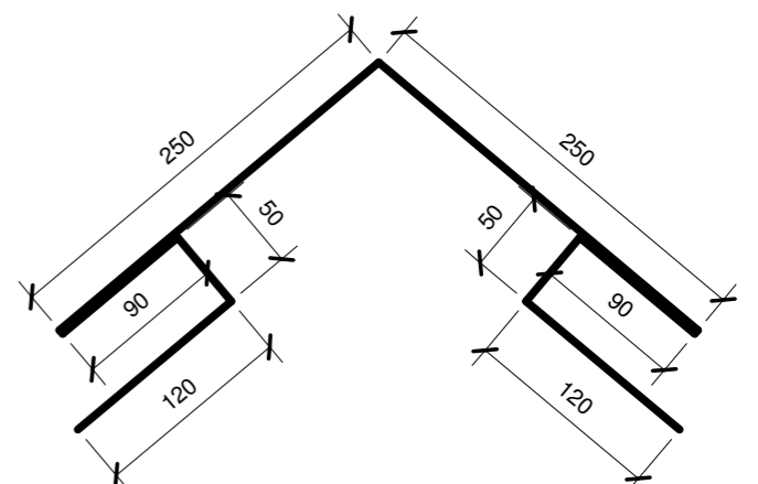
RIDGING FOR ROOF PITCH OVER 40 DEGREES ONLY
