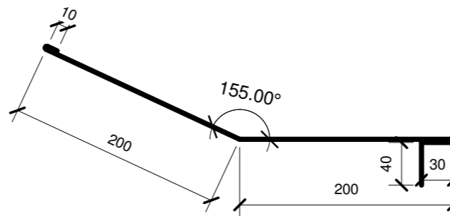
CHANGE OF PITCH
